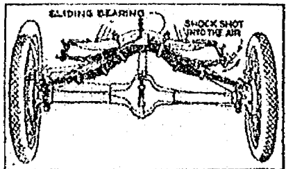
Illustrating Action of New Rear-Spring System When Left Wheel of Car Strikes an Obstruction, Shock Being Deflected to Right.
